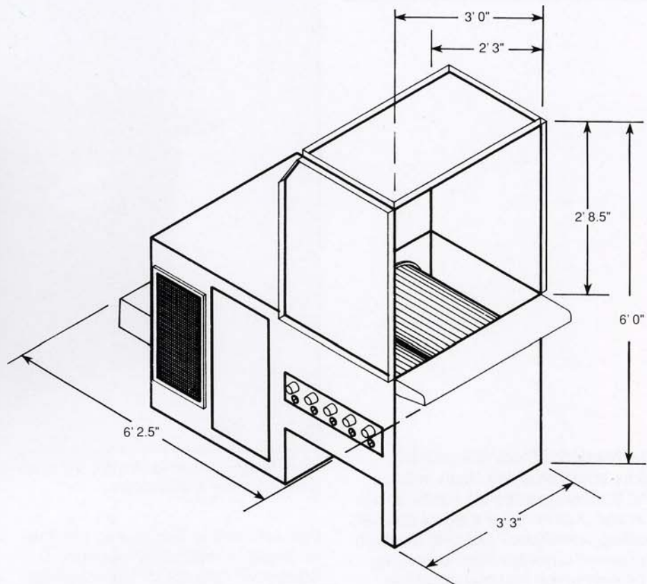
The Model 902 booth can be customized to accommodate varying automatic spray applications.
